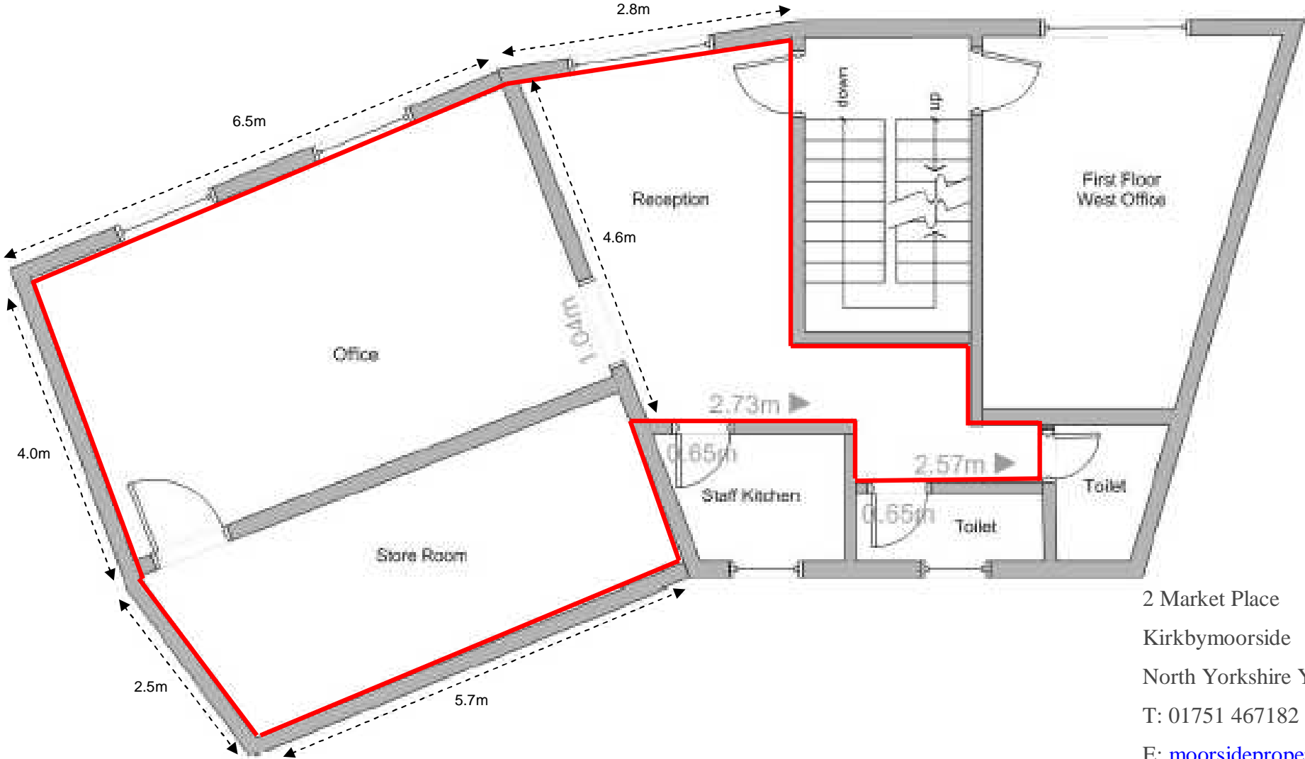
1 st Floor Office / Retail Space East: Plan
